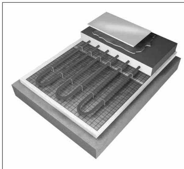
Rys. 42. KISAN COMFORT FLOOR STANDARD
